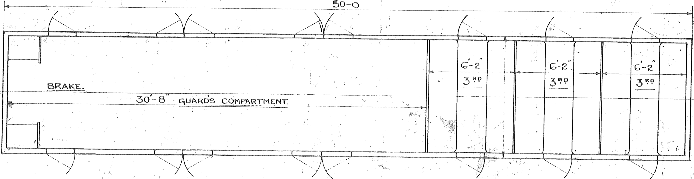
C.L.C. BOGIE THIRD CLASS AND BRAKE CARRIAGE.
